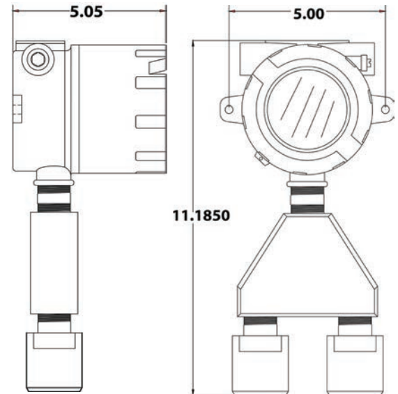
Dual Sensor Aluminum Housing
