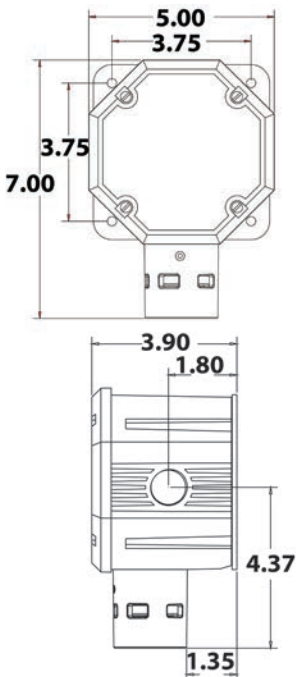
Poly Housing
